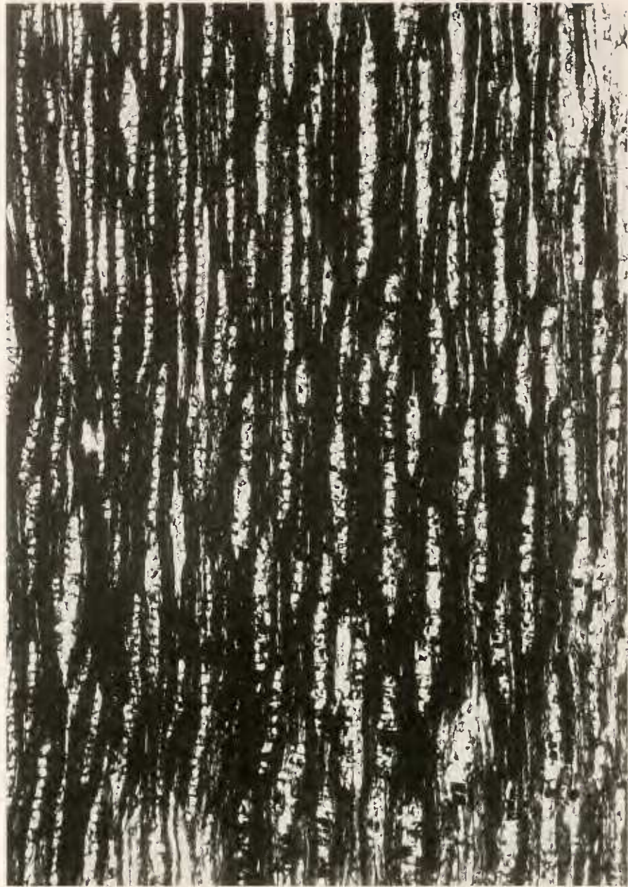
Fig. 7. Tangential longitudinal section through the secondary xylem showing homocellular rays. x 55
